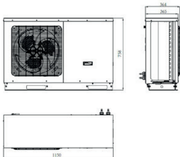
CH-HP4.0MIRK - CH-HP8.0MIRK
