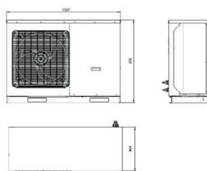
CH-HP10MIRM - CH-HP16MIRM
