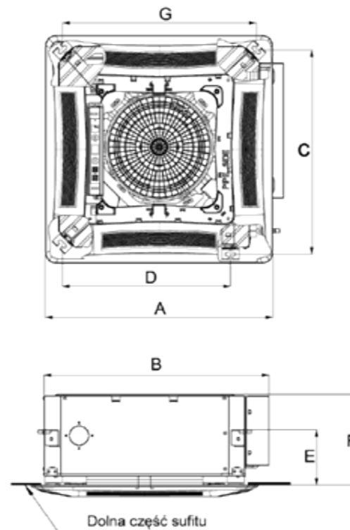
CHML-IC12RK CHML-IC18RK
